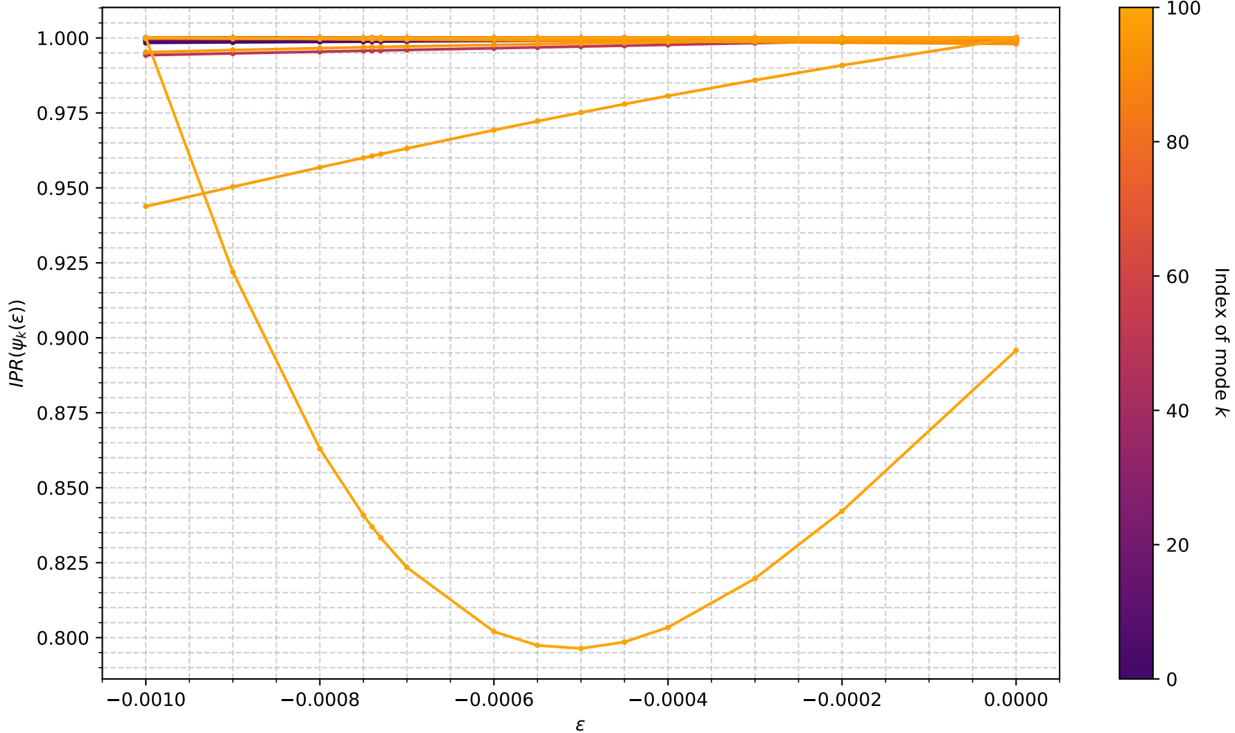
Normalized IPR for all modes, \gamma = 0.5
