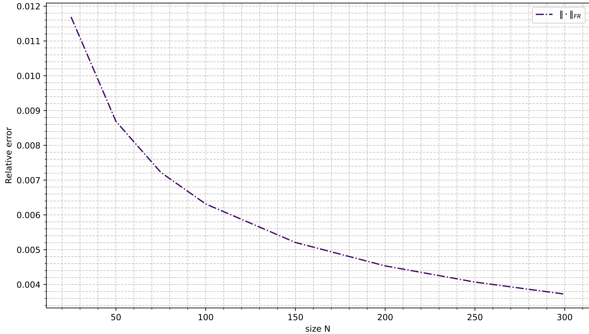
Toeplitz approximation error
