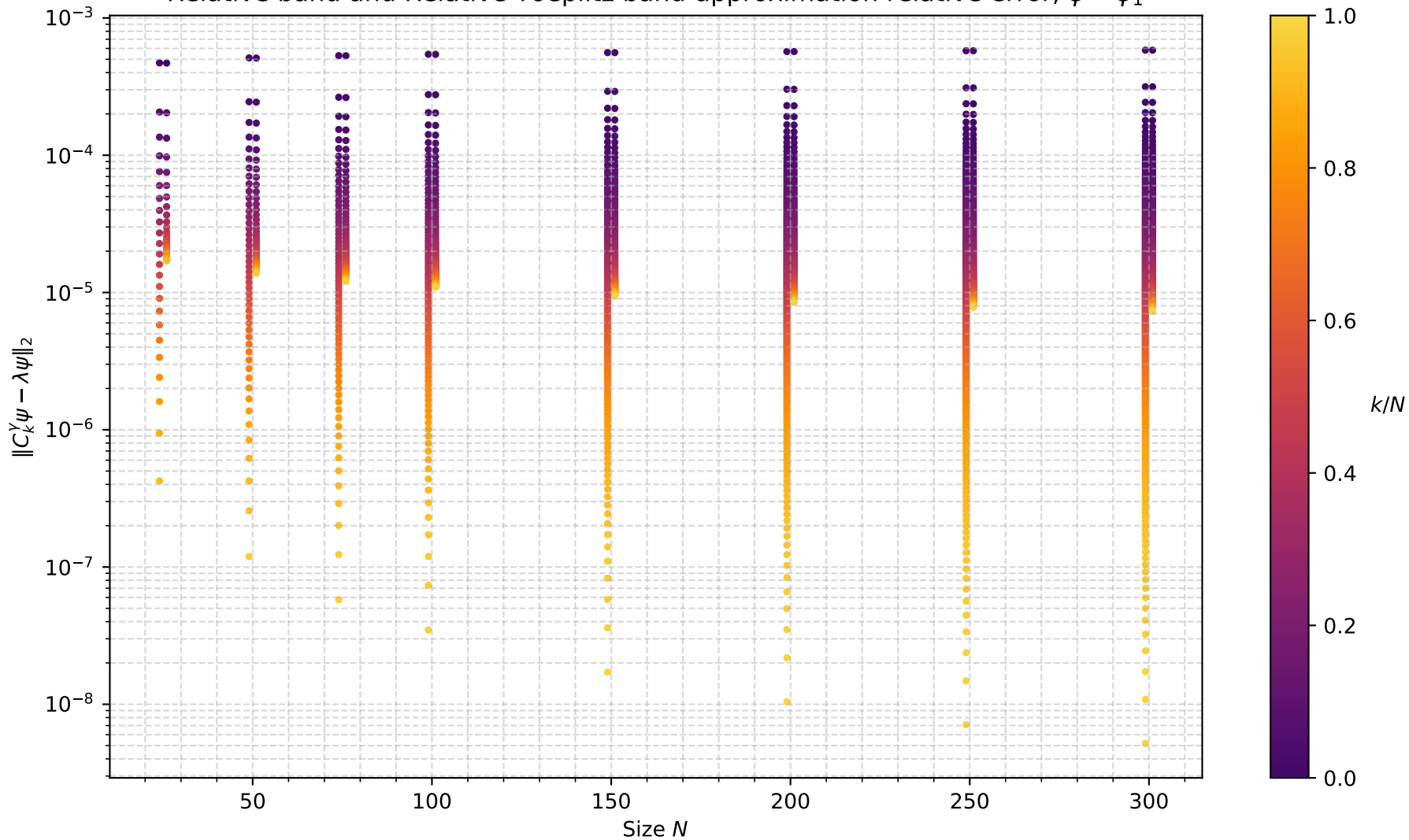
Relative band and Relative Toeplitz band-approximation relative error, \psi = \psi_1
