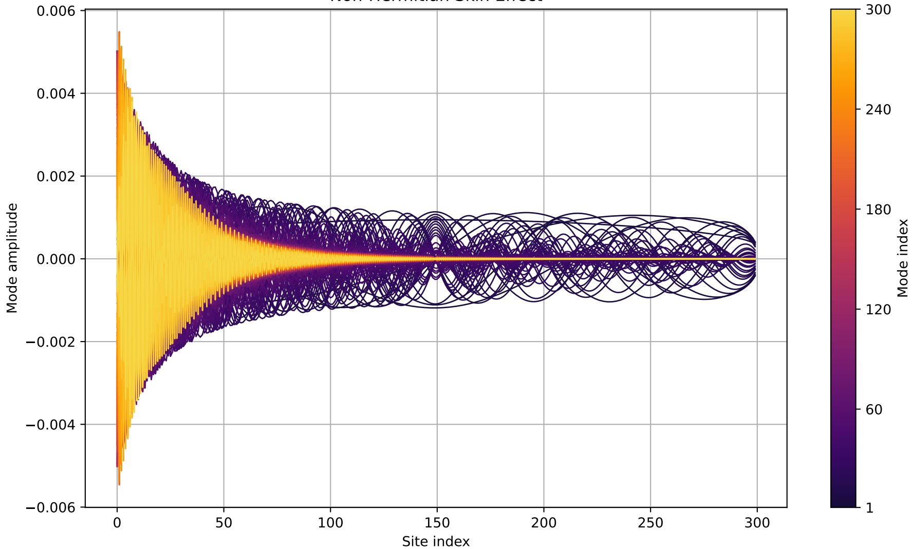
Non-Hermitian Skin Effect
