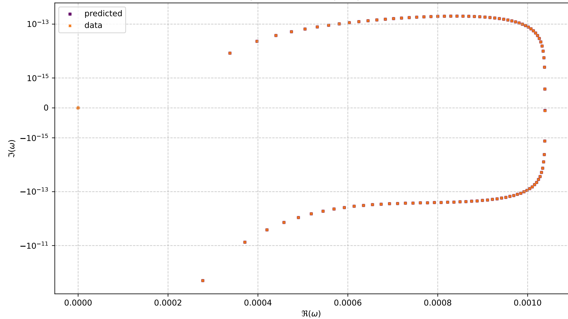
Eigenvalues in complex plane
