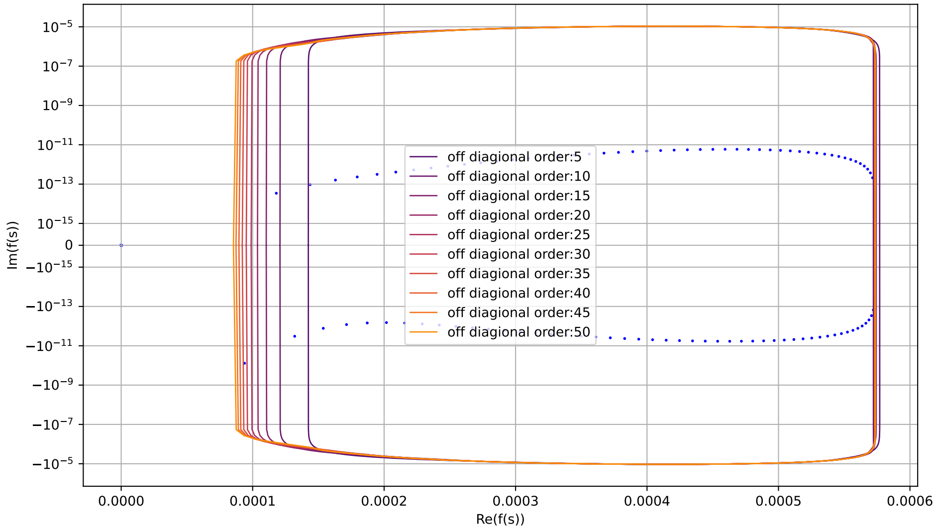
Winding regions for R = 0.3 skin GCM
