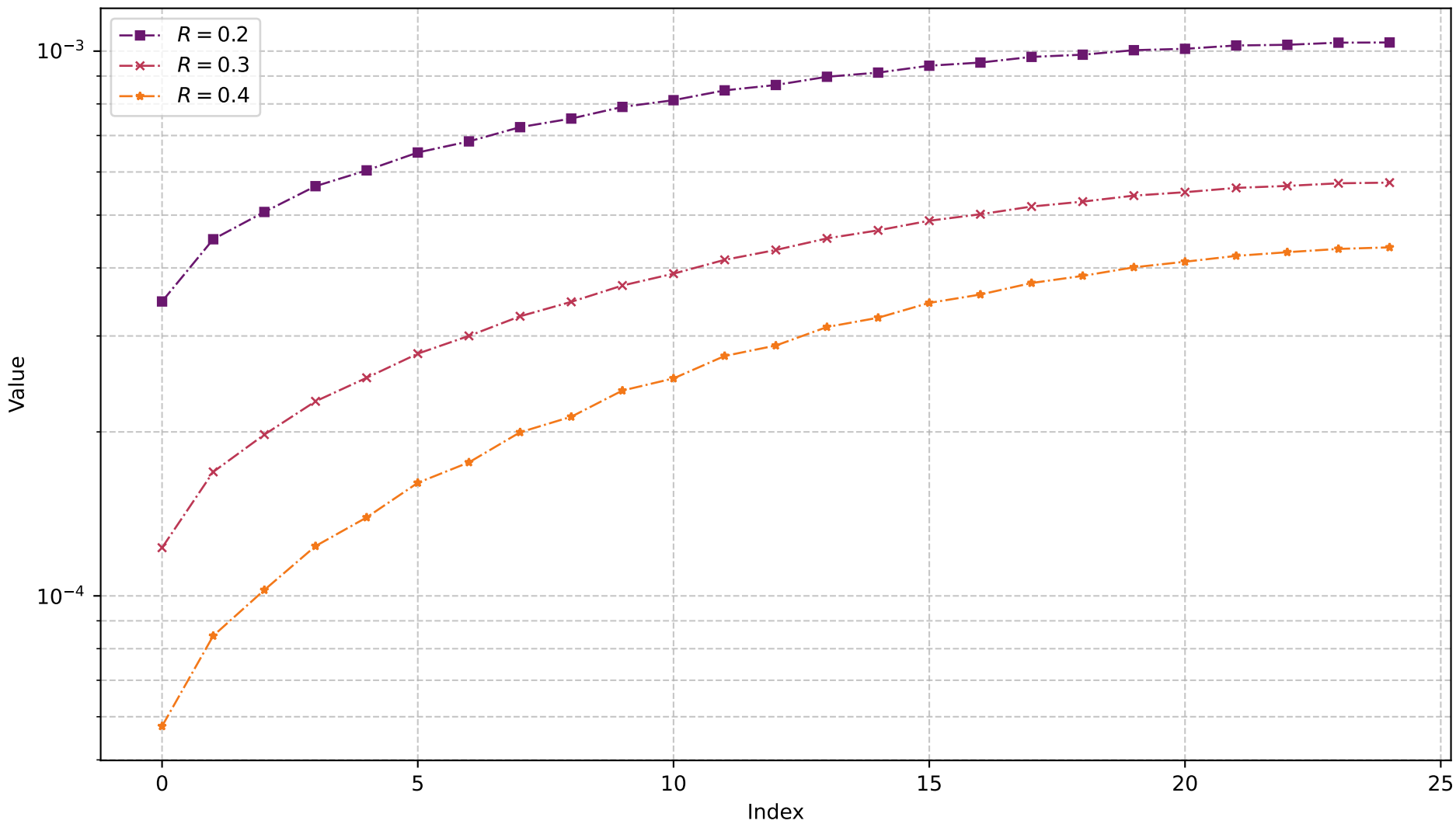
Real Frequencies N = 25 , \varepsilon = +0.01
