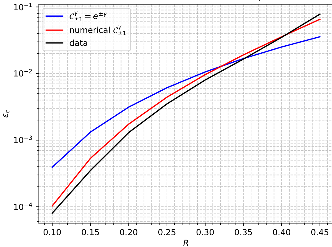
Defect threshold \varepsilon_c at first order, \gamma = 1
