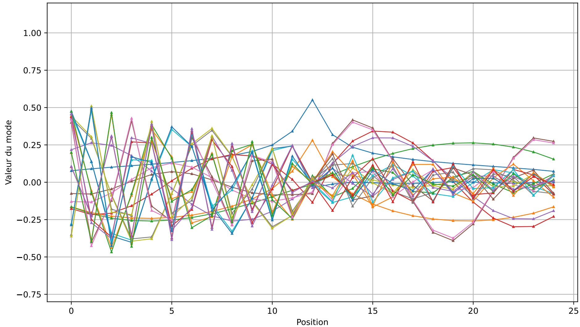
Modes R = 0.2 , \varepsilon = +0.1
