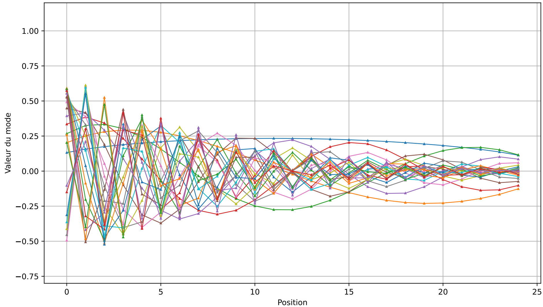
Modes R = 0.3 , \varepsilon = 0.0
