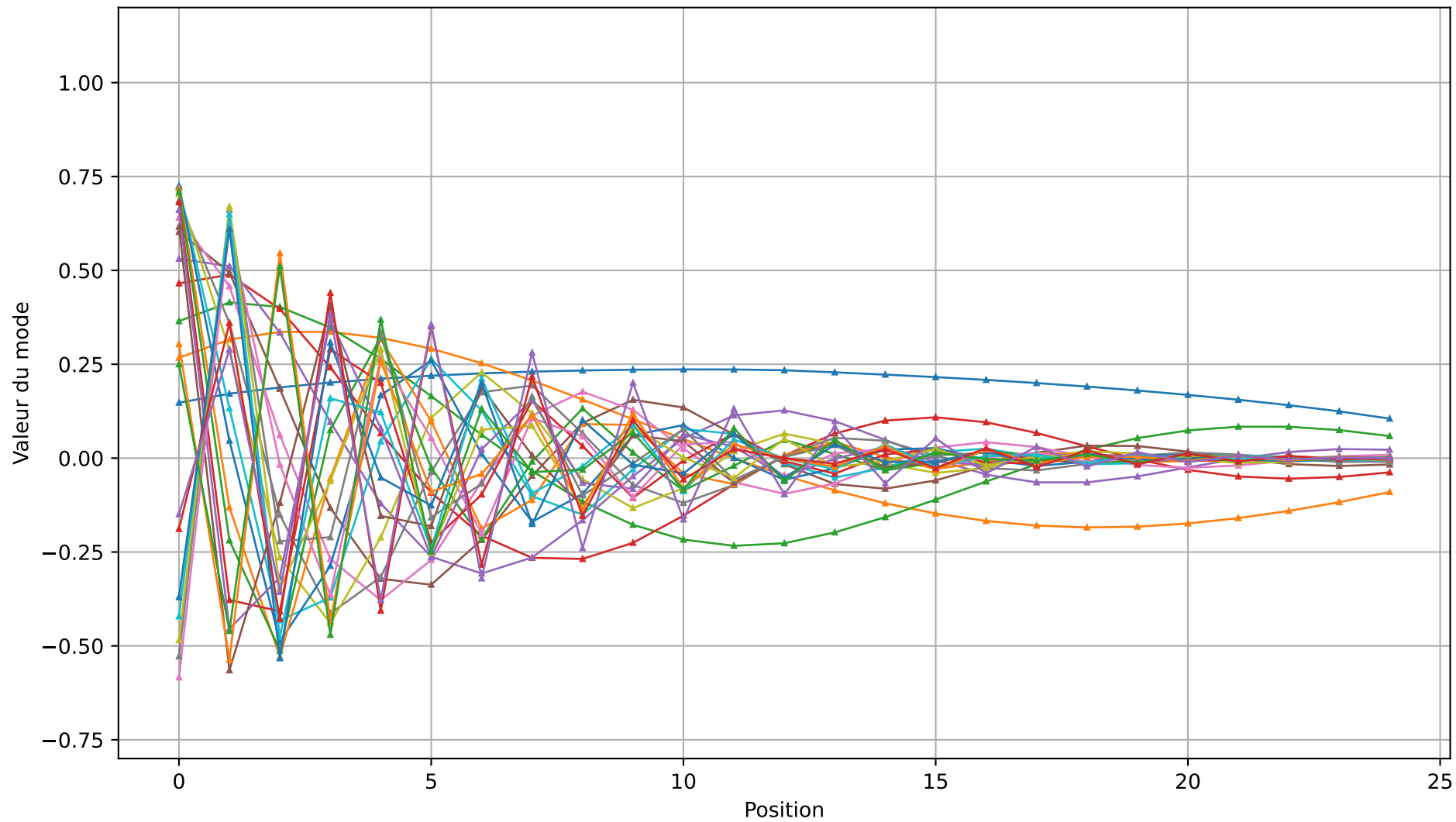
Modes R = 0.4 , \varepsilon = +0.01
