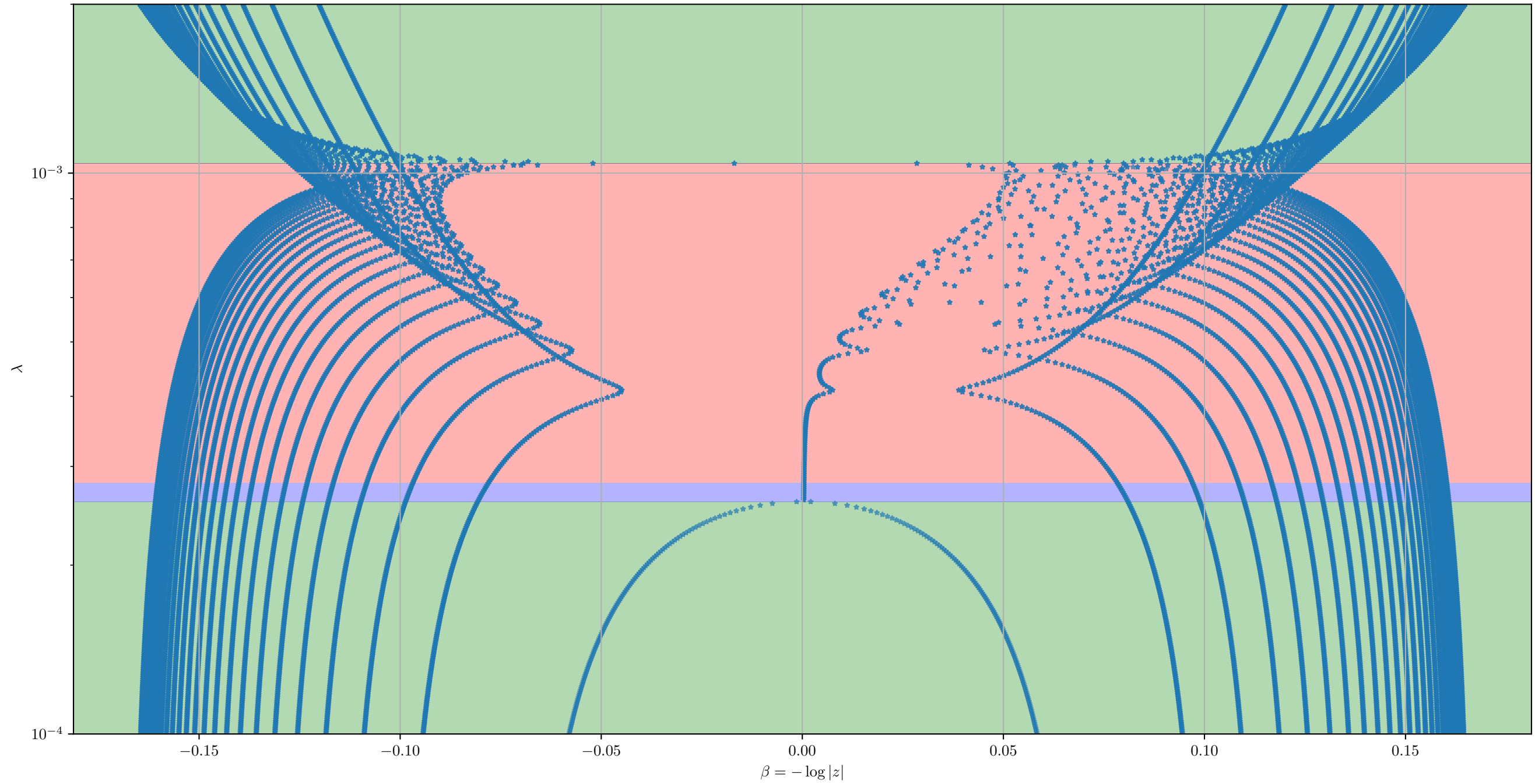
Complex band structure (beta vs lambda)
