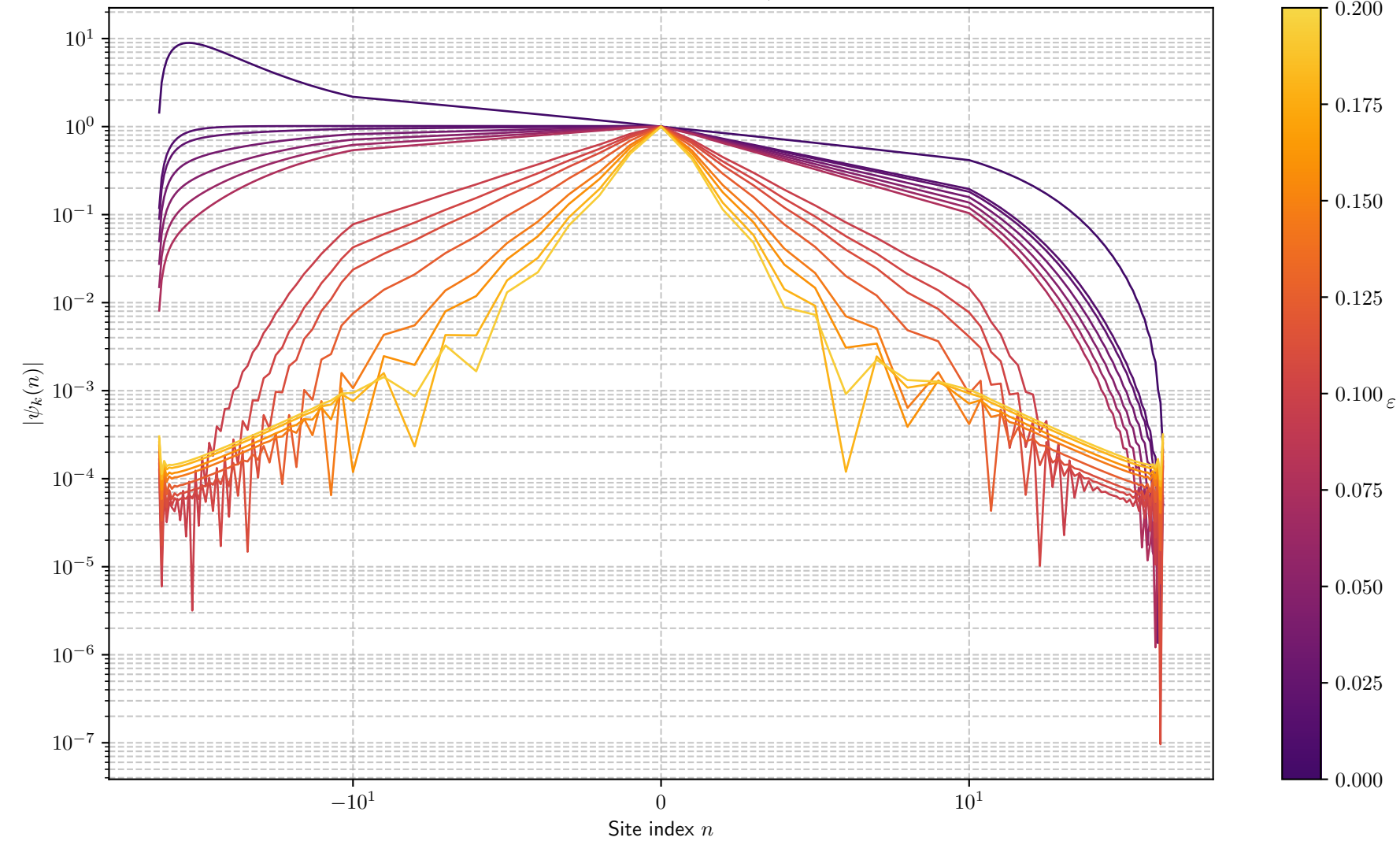
Positive defect, mode \psi_0
