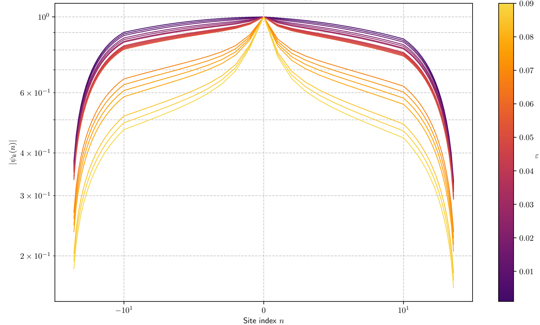
Positive defect, mode \psi_0
