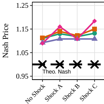
Hotelling
