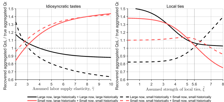
Figure 2b: Total error after aggregation
