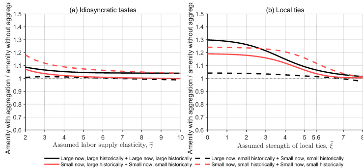
Figure 2c: Pure aggregation error
