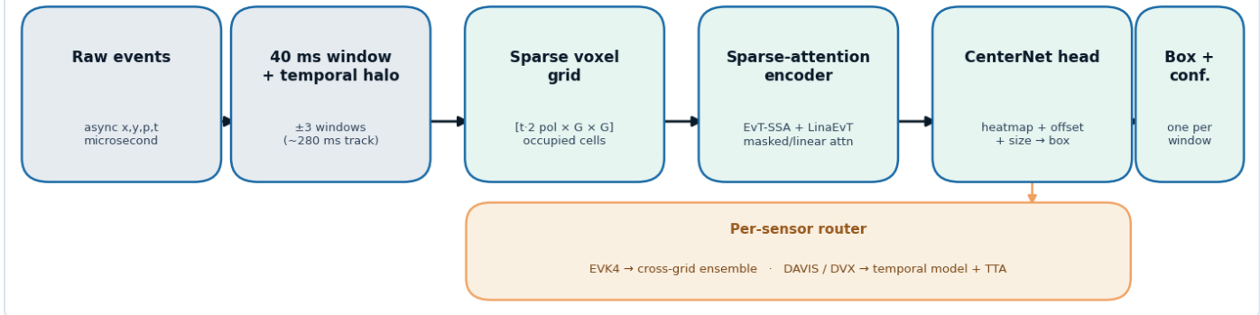
Fig 1 — End-to-end pipeline: raw asynchronous events → windowed sparse voxel grid → sparse-attention encoder → CenterNet head, with a per-sensor router selecting the best detector for each sensor.
