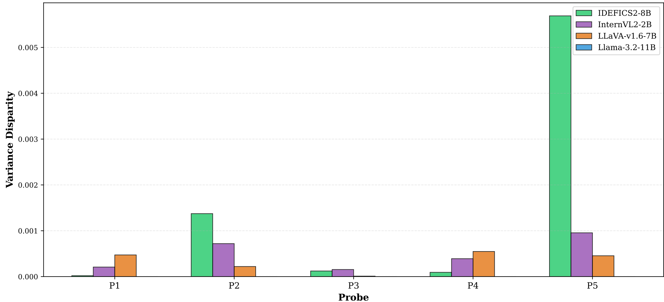
Variance Gaps by Probe
