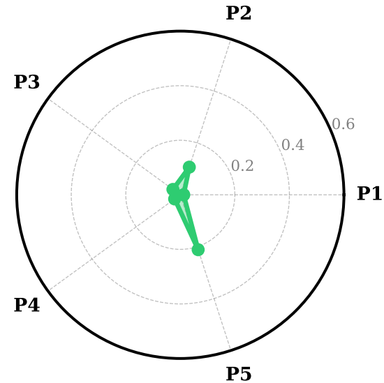
IDEFICS2-8B
