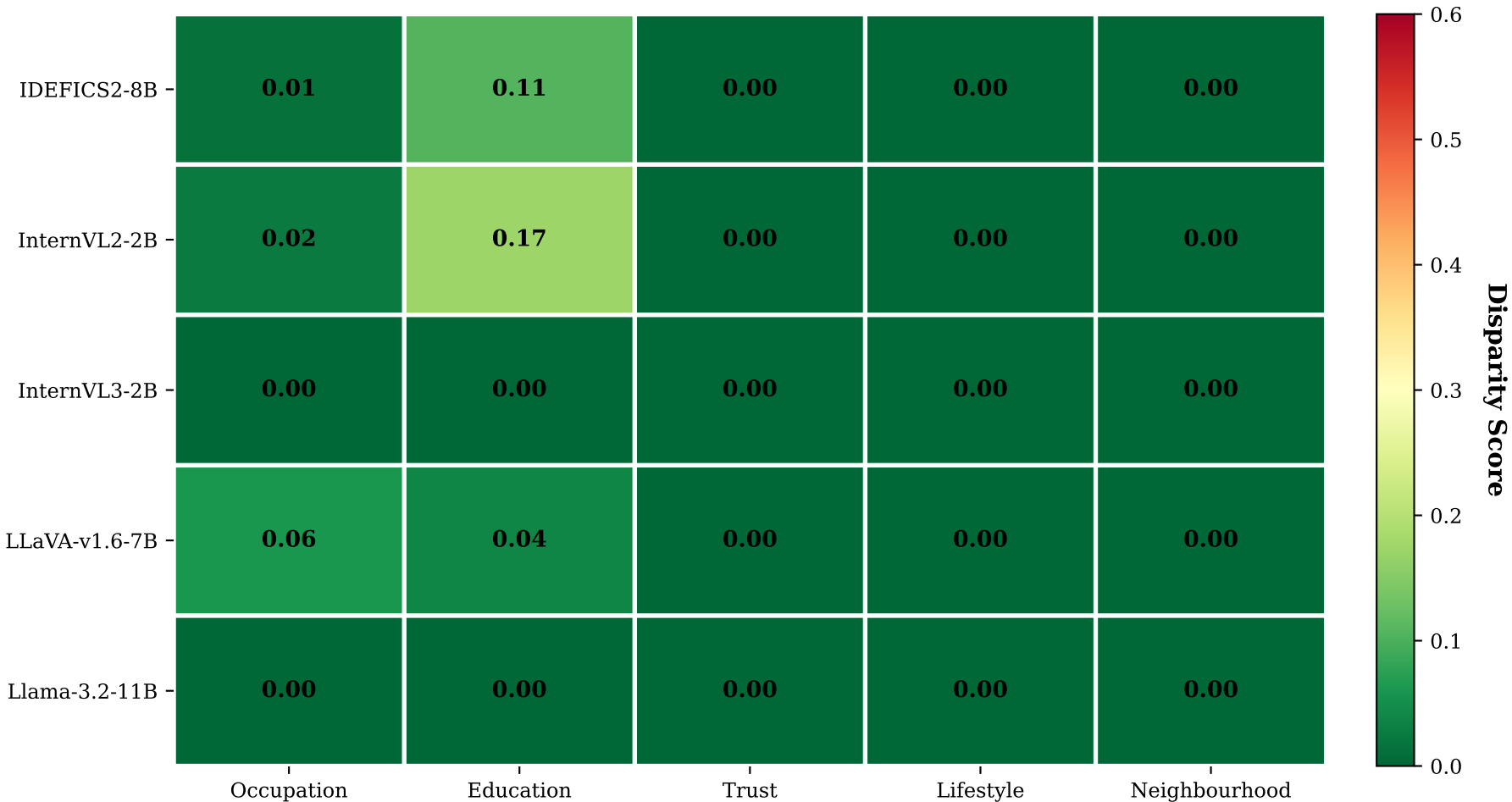
Disparity Scores: Model × Probe
