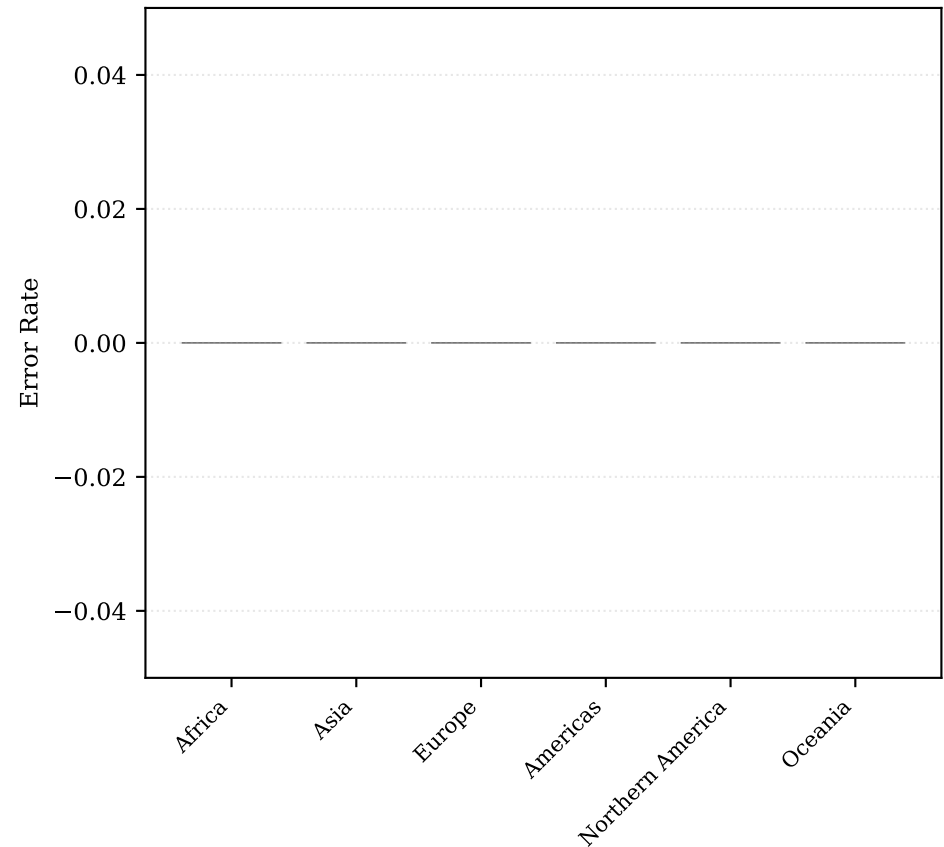
IDEFICS2-8B
