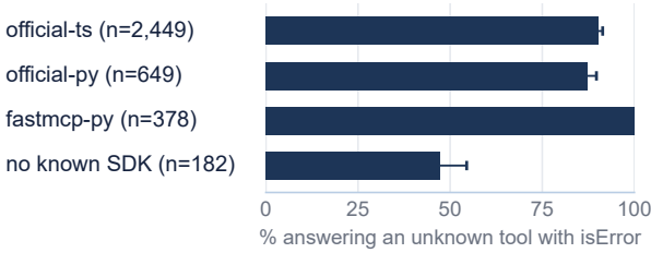
Fig. 4. Unknown-tool responses by SDK family. In every family, most servers answer with an isError result. Bars show 95% Wilson intervals; families with fewer than 25 servers appear in Table IV only.
