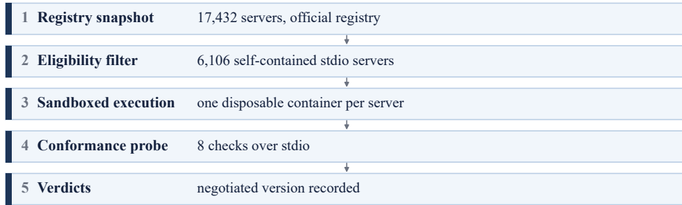
Fig. 1 Measurement pipeline. Every eligible server is installed and executed in its own disposable container, then driven through the conformance probe. The protocol version each server negotiates is recorded with its verdicts, and no check depends on it.
