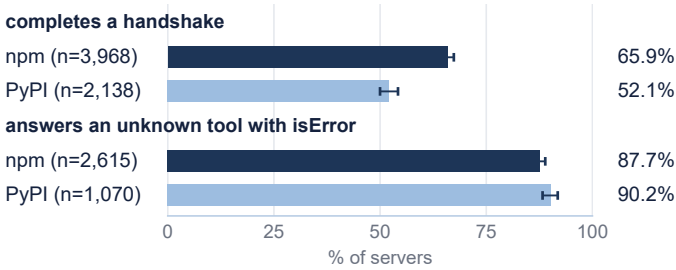
Fig. 5. Handshake yield (PyPI after the entry-point correction) and the error-as-result rate for unknown tools, by package registry, with 95% Wilson intervals.
