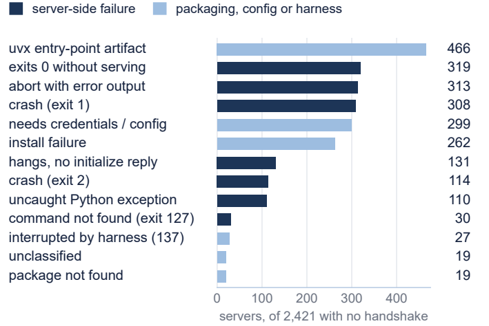
Fig. 2. Why servers never reach a handshake. Configuration requirements and the entry-point artifact are separated from genuine startup failures.
