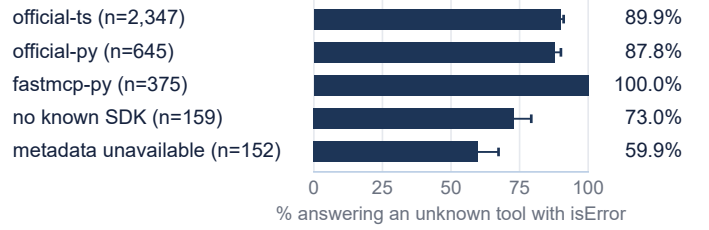
Fig. 4. Unknown-tool responses by SDK family. In every family, most servers answer with an isError result. Bars show 95% Wilson intervals; families with fewer than 25 servers appear in Table IV only.
