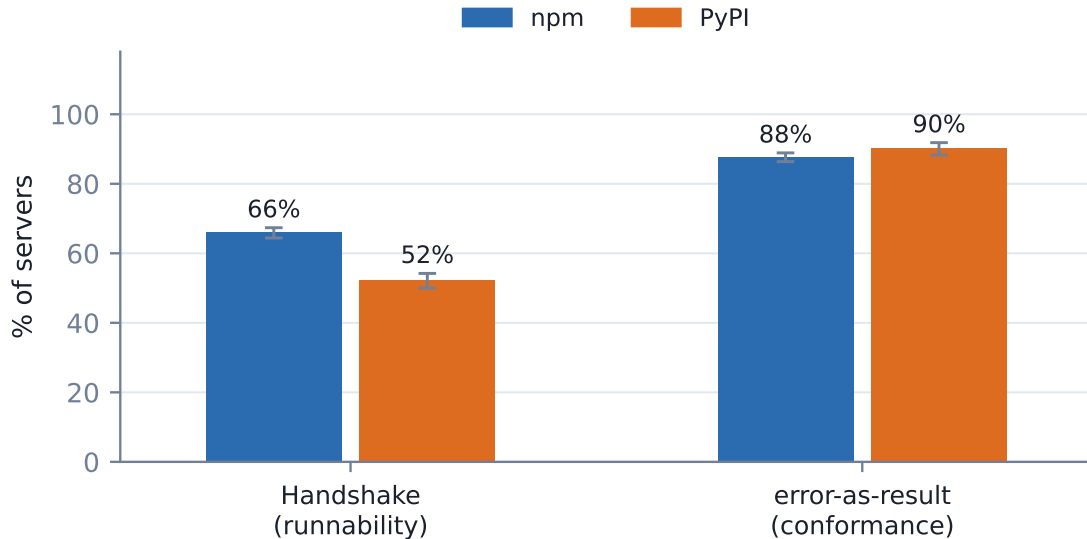
Figure 5: Handshake yield and conformance-check pass rates by package registry, with 95% confidence intervals.
