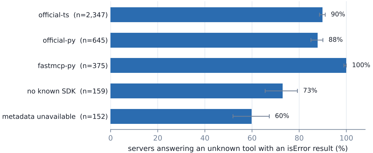
Figure 4: Which mechanism a server uses tracks its SDK, not its author. Every SDK family answers an unknown-tool call with an isError result rather than a protocol error in the large majority of cases. Bars show 95% Wilson intervals; families with fewer than 25 servers appear in Table 4 only.
