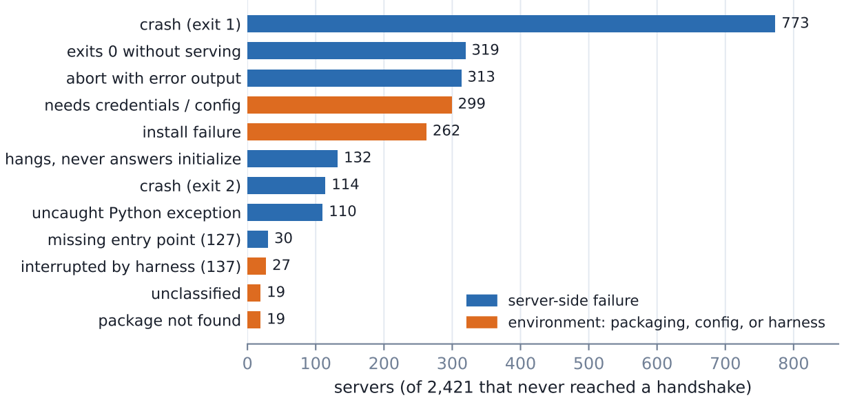
Figure 2: Why servers never reach a handshake. Configuration requirements and the entry-point artifact are separated from genuine startup failures.
