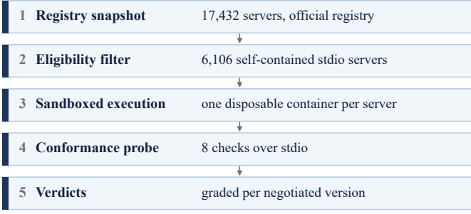
Fig. 1. Measurement pipeline. Every eligible server is installed and executed in its own disposable container, then driven through the conformance probe. The protocol version each server negotiates is recorded with its verdicts, and no check depends on it.
