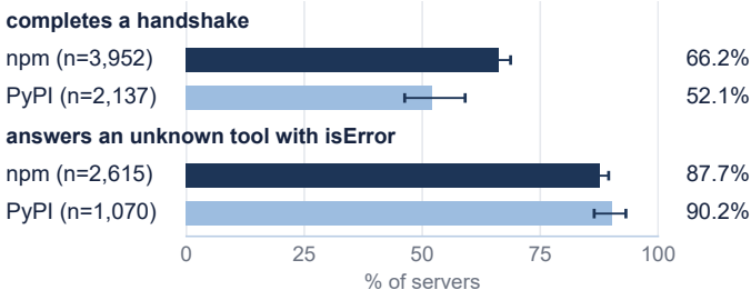
Fig. 5. Handshake yield (PyPI after the entry-point correction) and the error-as-result rate for unknown tools, by package registry, with 95% intervals from a publisher-cluster bootstrap.
