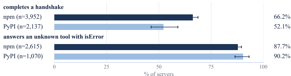
Fig. 5 Handshake yield (PyPI after the entry-point correction) and the error-as-result rate for unknown tools, by package registry, with 95% intervals from a publisher-cluster bootstrap.
