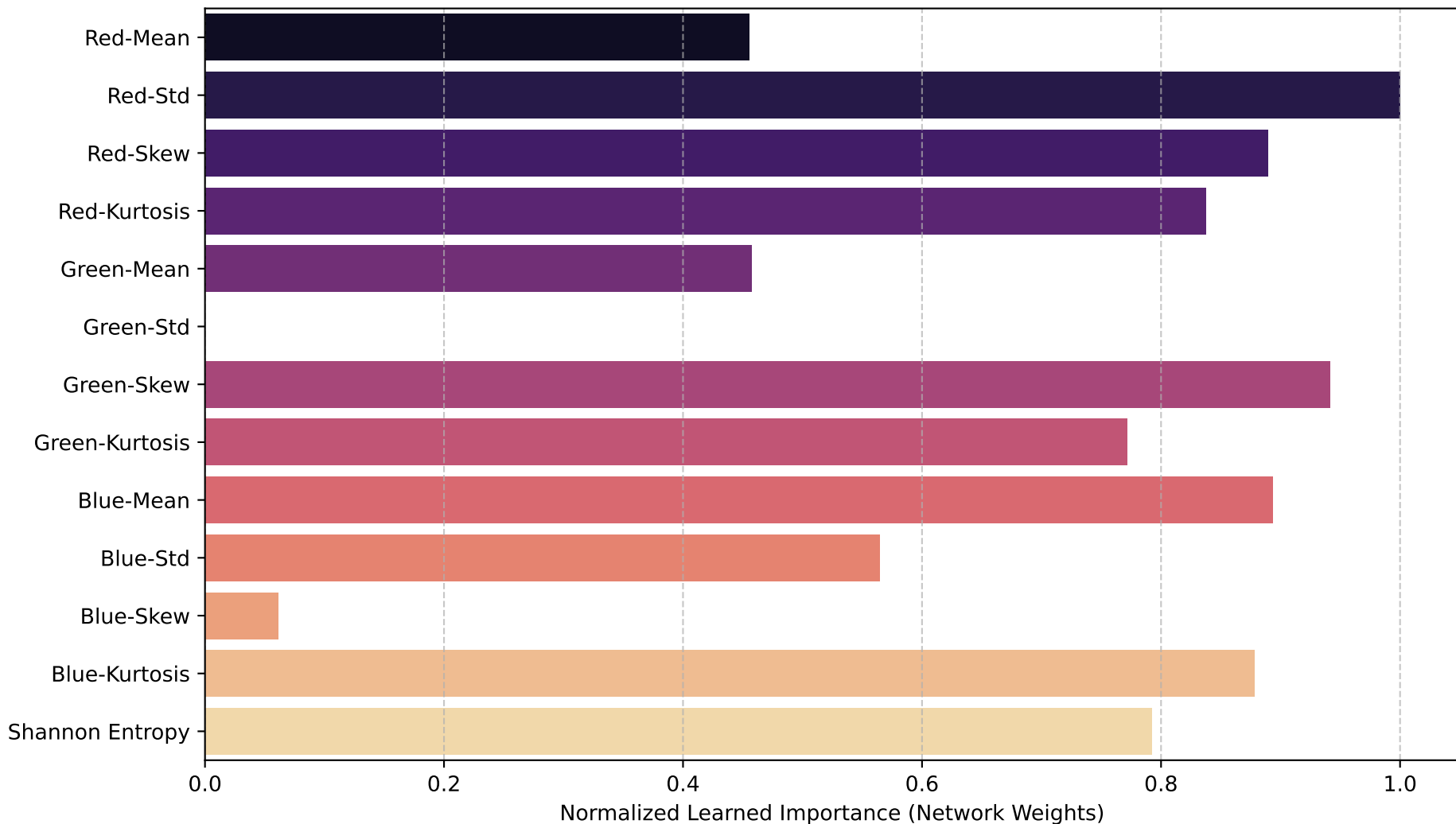
XAI: Pathology Statistical Feature Importance (Global Weight Attribution)
