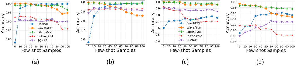
Fig. 2. Performance of few-shot fine-tuning for Wave2Vec2BERT and HuBERT with a varying number of few-shot audio samples from OpenAI and Seed-TTS, respectively. (a) Fine-tune Wave2Vec2BERT on OpenAI; (b) Fine-tune HuBERT on OpenAI; (c) Fine-tune Wave2Vec2BERT on Seed-TTS; and (d) Fine-tune HuBERT on Seed-TTS.
