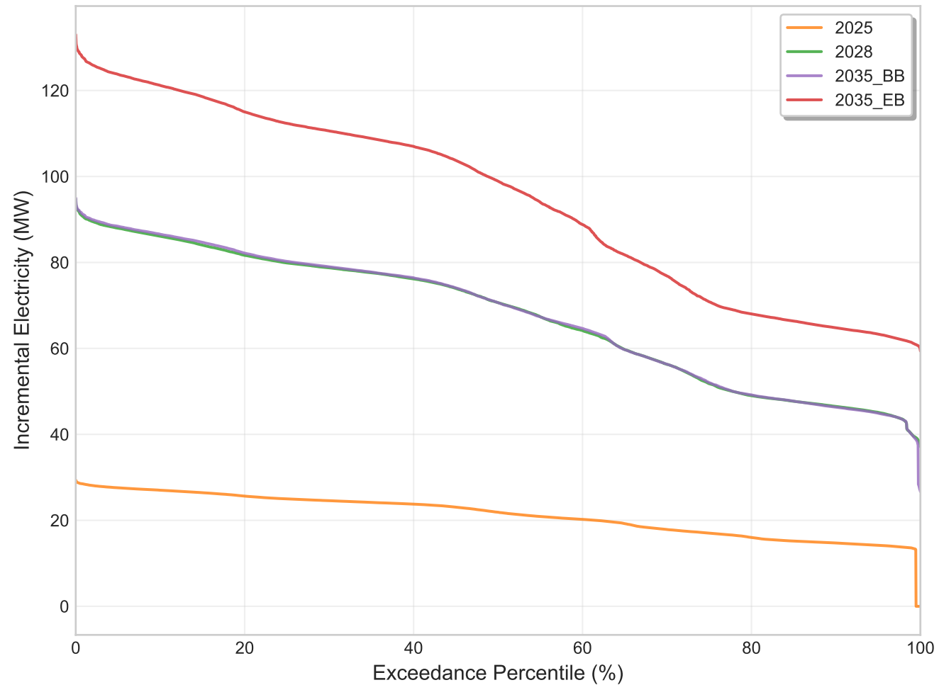
Duration Curves: Incremental Electricity Across Epochs
