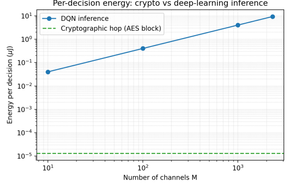
Figure 7: Per-decision energy: crypto vs DL.
