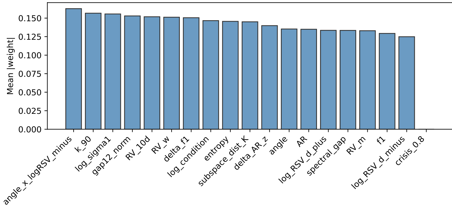
Feature importance (DNN HAR+SVD, first layer)
