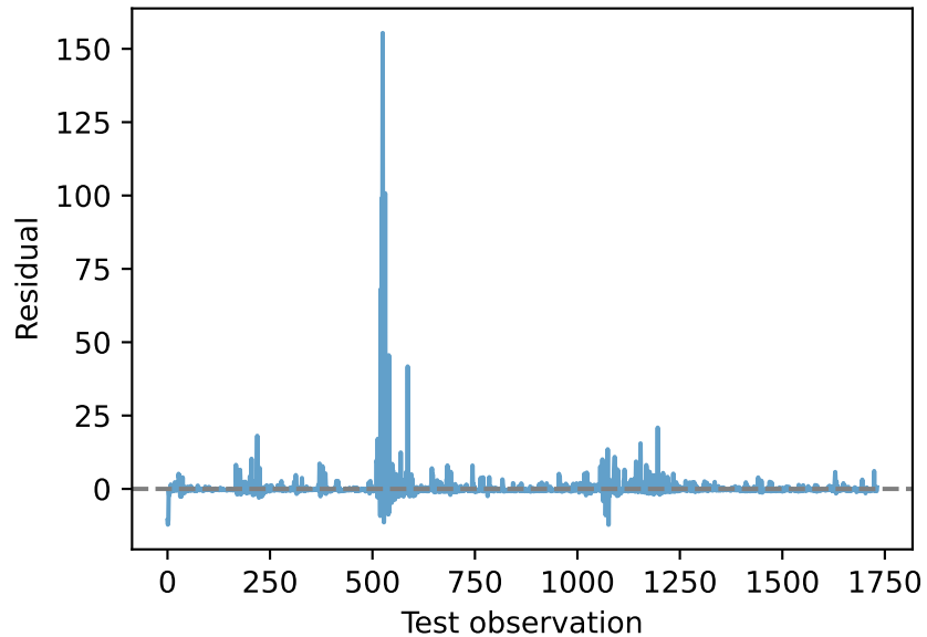
Residuals over time (DNN_HAR+SVD)
