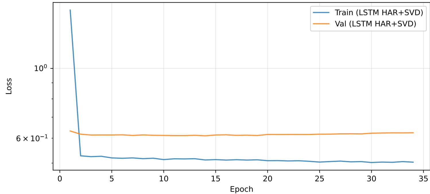
Training loss curves (LSTM HAR+SVD)
