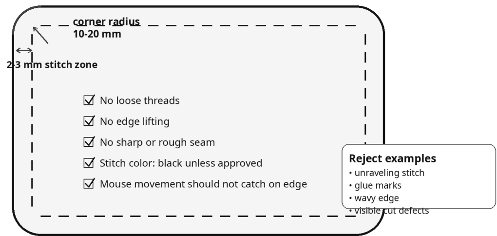
Figure 3 - Stitched edge and rounded corner detail
