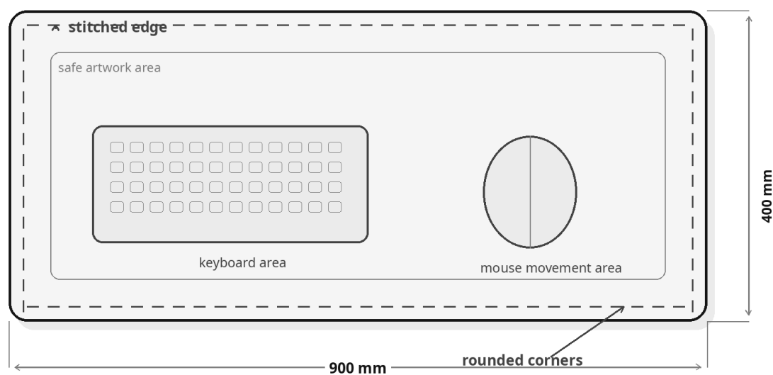
Figure 1. Target product overview and main dimensions.
