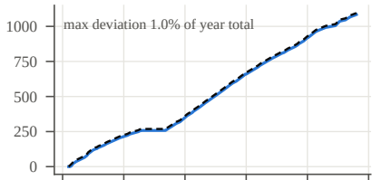
fraud 2
