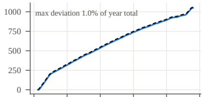
fraud 3
