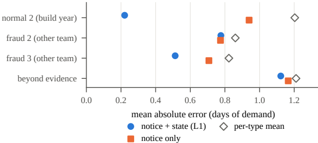
(a) impact prediction error
