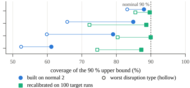
(b) conformal coverage under shift
