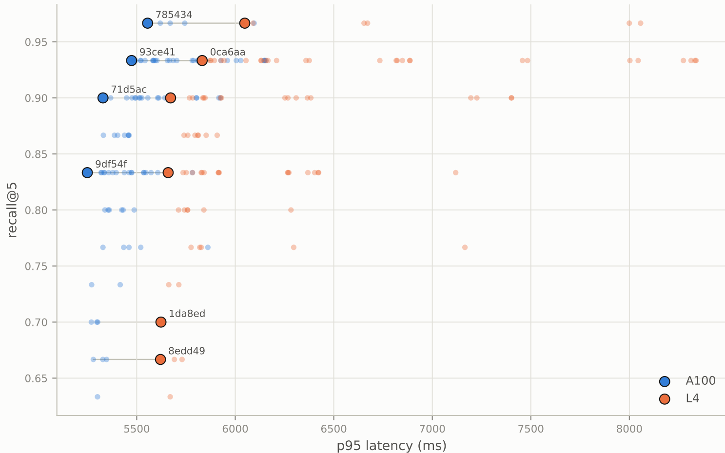
Figure 1 — recall@5 vs p95 latency, A100 vs L4 filled = on that card's Pareto frontier; thin lines trace one config across cards
