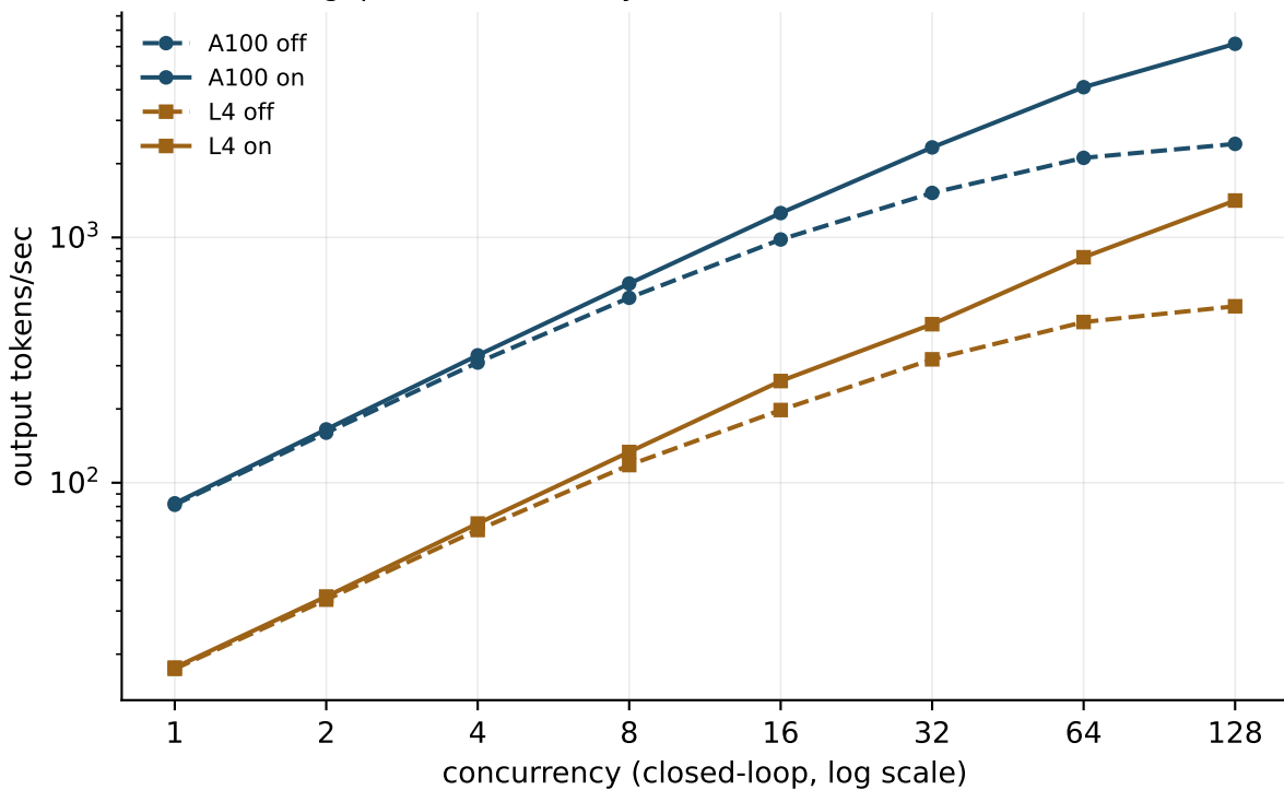
Throughput vs concurrency — vLLM, Qwen2.5-7B-Instruct, FP16
