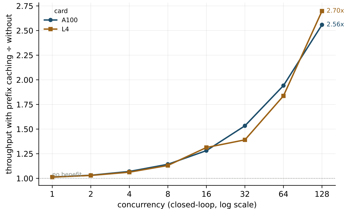
The payoff from prefix caching transfers across hardware tiers
