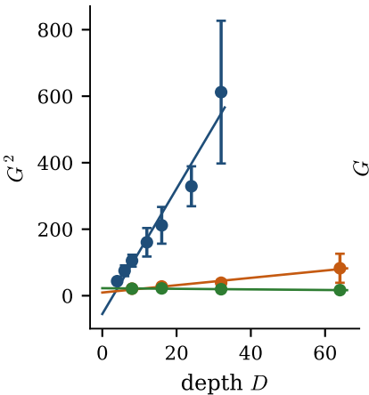
(a) MLPs: G^2 grows with D
