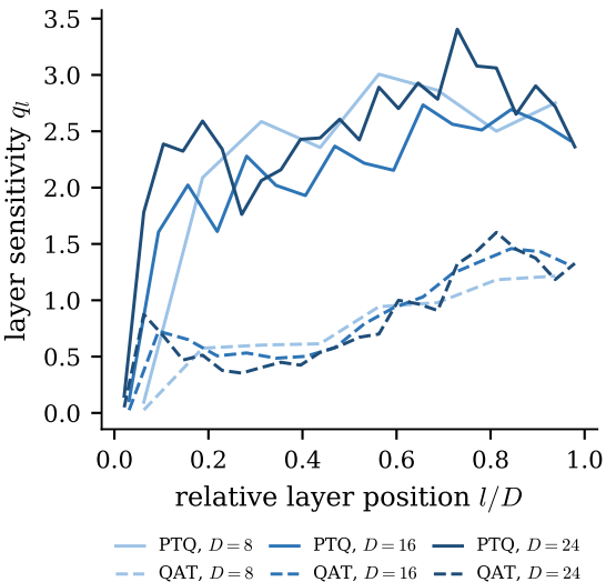
(a) QAT lowers every layer's sensitivity
