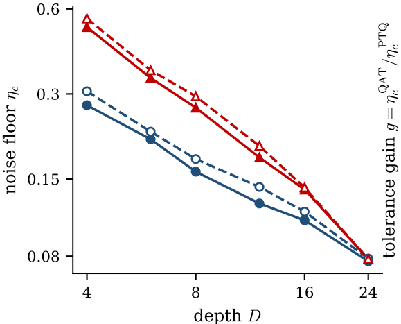
(a) plain MLP: QAT higher but steeper
