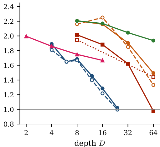
(b) QAT benefit decays with depth
