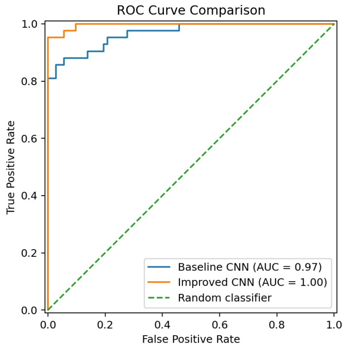
Figure 4. ROC curve comparison on the untouched test set.
