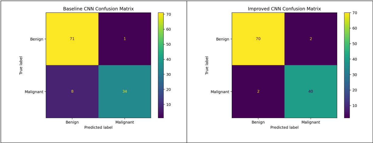
Figure 3. Baseline confusion matrix (left) and improved confusion matrix (right).
