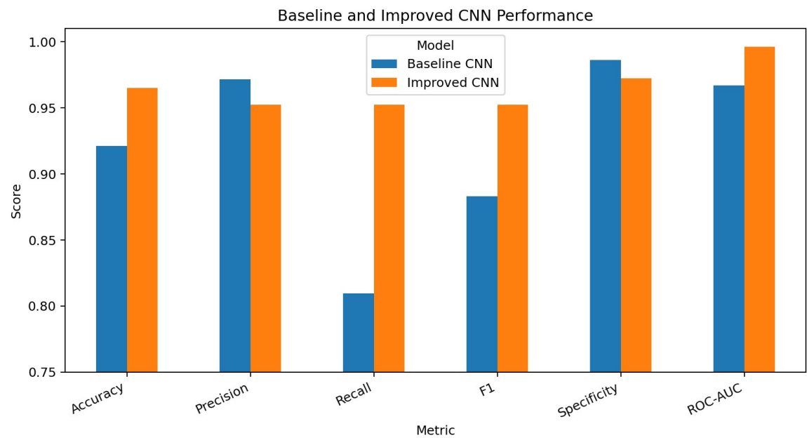
Figure 2. Comparison of baseline and improved model metrics.
