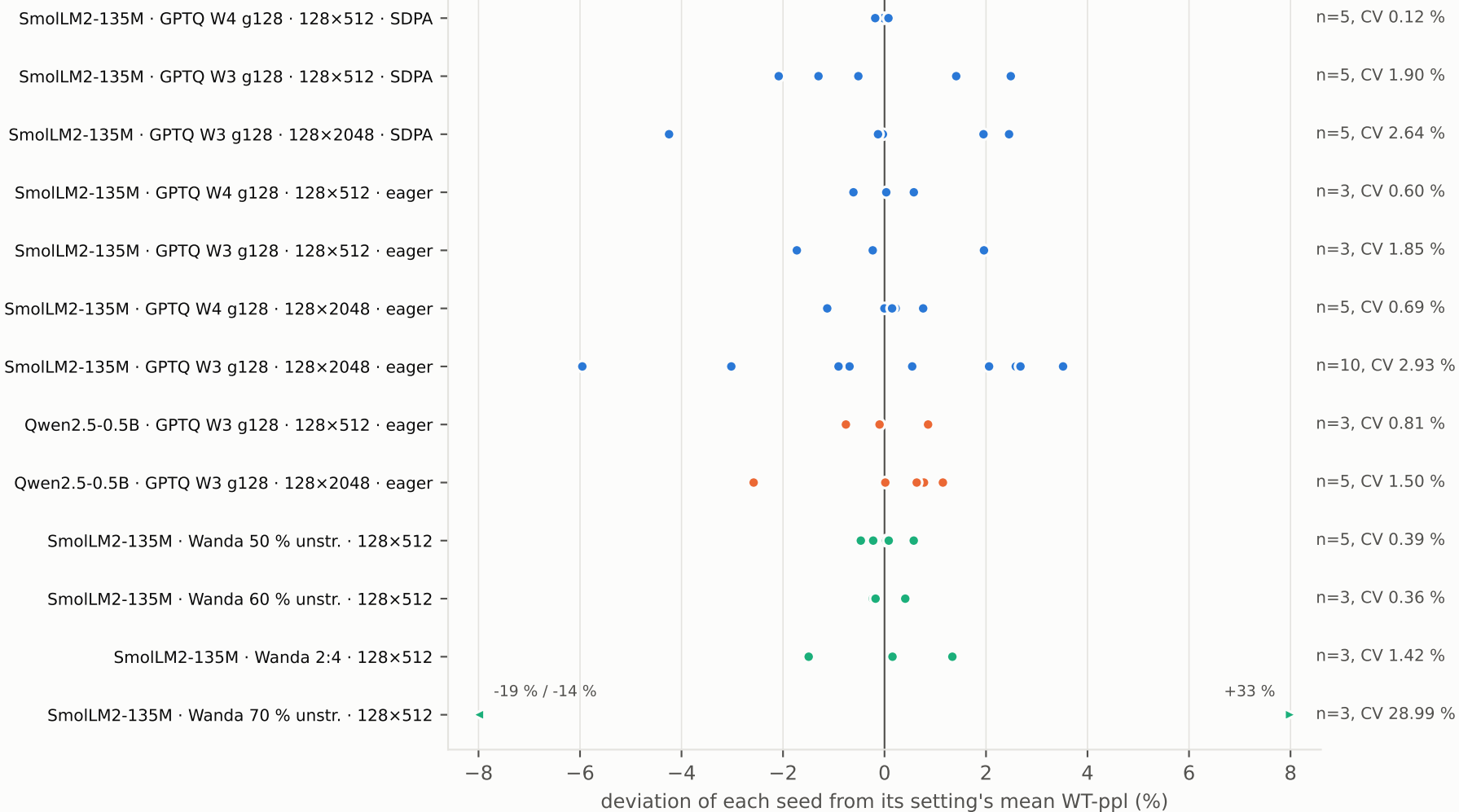
Calibration-seed spread per setting (blue: GPTQ SmoLLM2, orange: GPTQ Qwen, aqua: Wanda)
