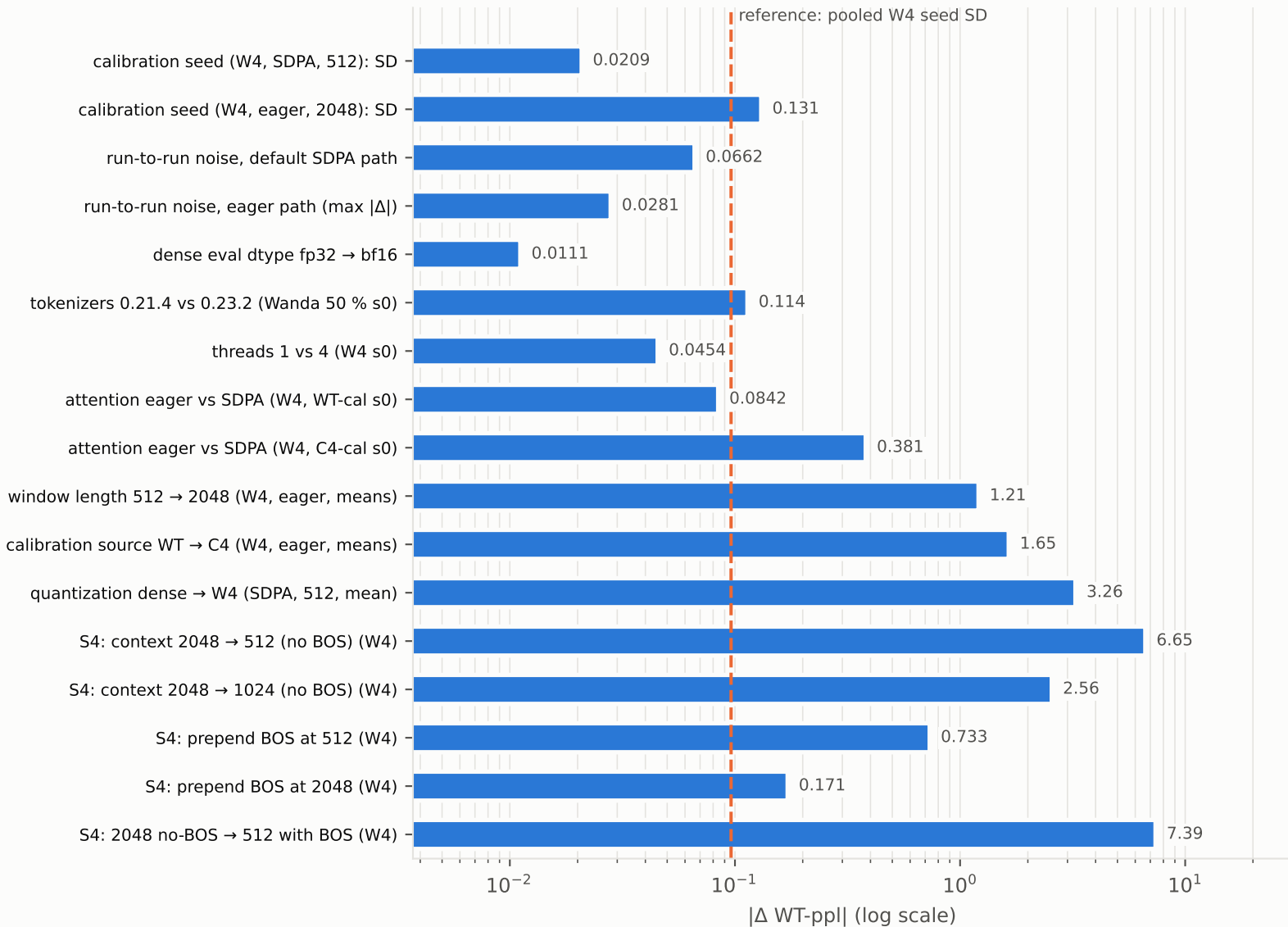
Size of protocol factors vs. the effect being reported (SmolLM2-135M)
