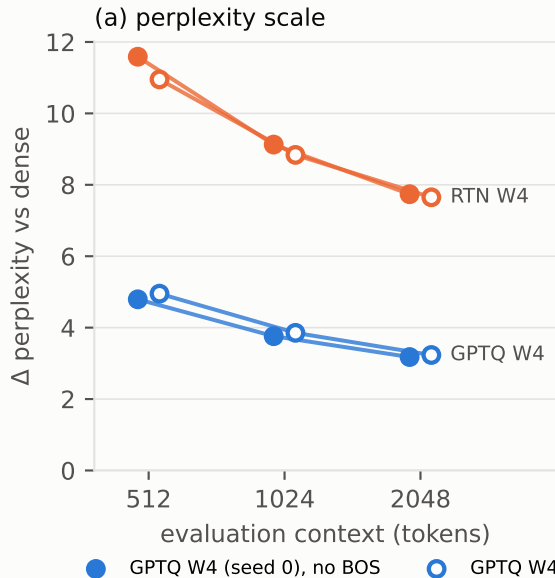
Damage of one W4 checkpoint under six perplexity protocols (SmolLM2-135M, same 81,920 WikiText-2 tokens)
