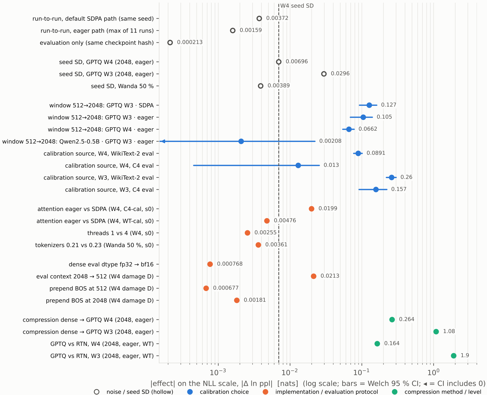
Synthesis: size of every measured factor on one scale (SmoLM2-135M unless noted)
