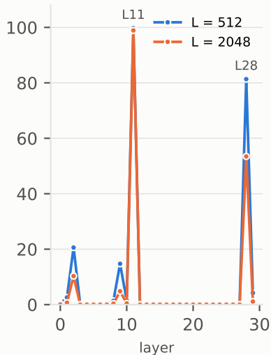
(b) SmolLM2-135M
