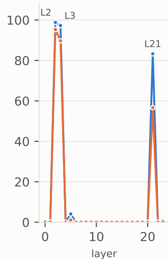
(c) Qwen2.5-0.5B
